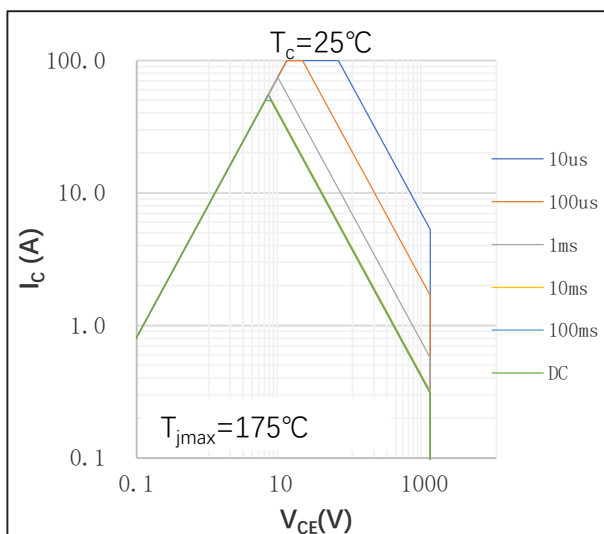
● Fig.11 Safe operating area: continuous and peak collector currents as a function of collector-emitter voltage; Calculative values
